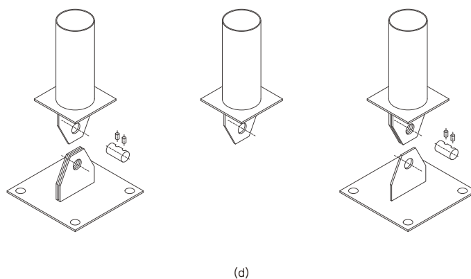
Some examples of tubular connections with pinned ends 帶銷端的管狀連接的一些示例
