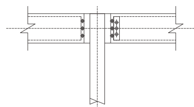
(a-3) C-sections welded to an RHS column to facilitate the use of a bolted connection 焊接在扁通柱上的C型鋼，以便使用螺栓連接
